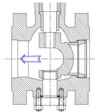
Shaft Downstream
