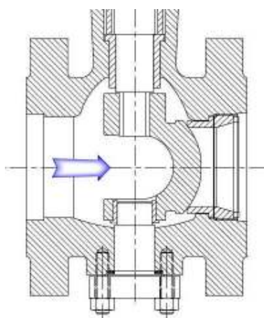
Shaft Upstream
