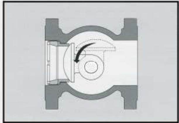
Valve Closing
